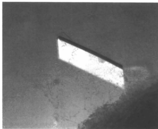
Fig. 1. Crystal of human AdoHcy hydrolase. The crystal is approximately 0.8 \times 0.25 \times 0.1 mm.
